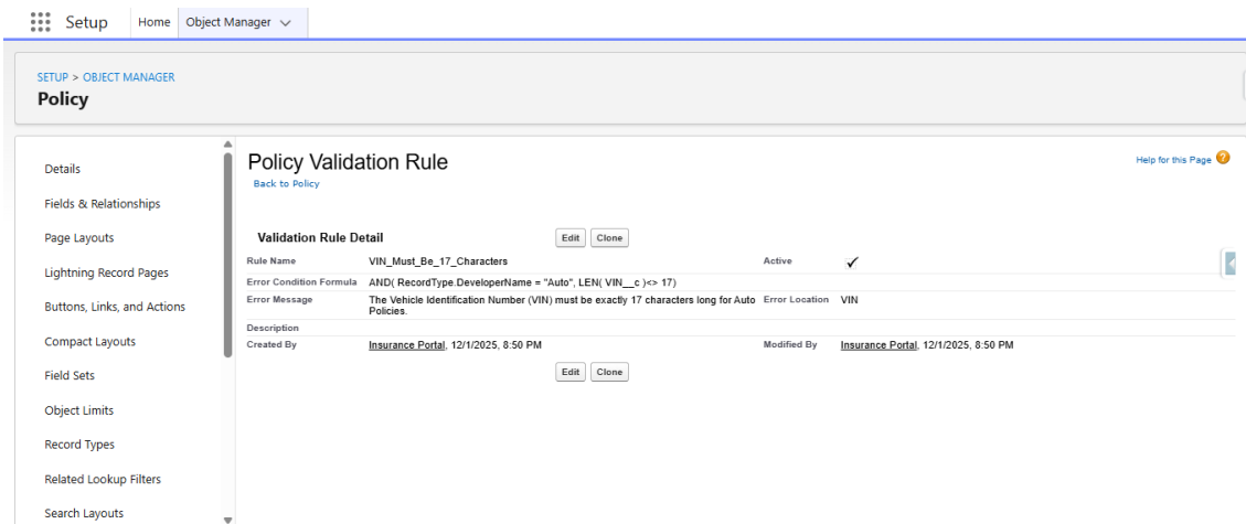
Figure 8: VIN_Must_Be_17_Characters validation rule
