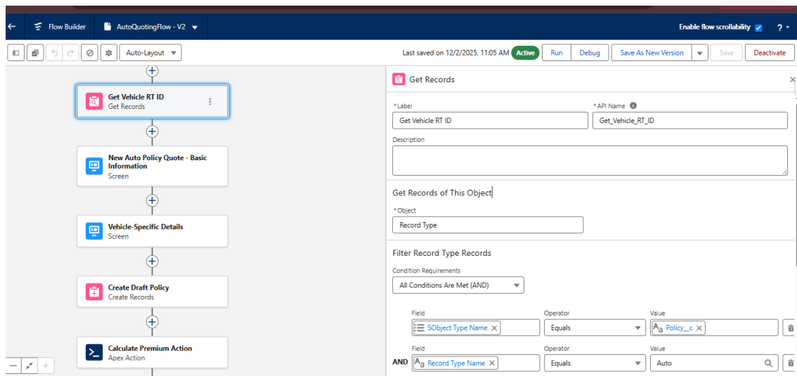
Figure 7: AutoQuotingFlow - Get Vehicle RT ID element
