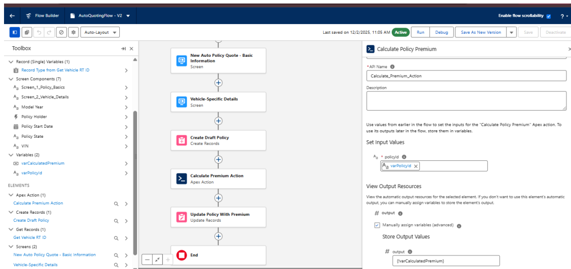
Figure 9: Calculate Premium Action in AutoQuotingFlow
